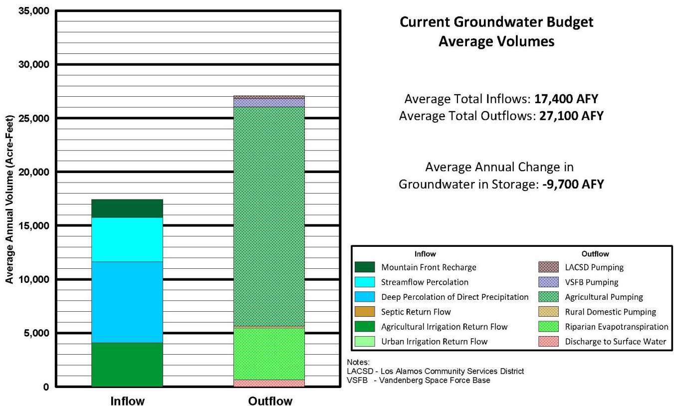
Figure 5-1. Updated Current Groundwater Budget (2011-2025) Average Volumes
